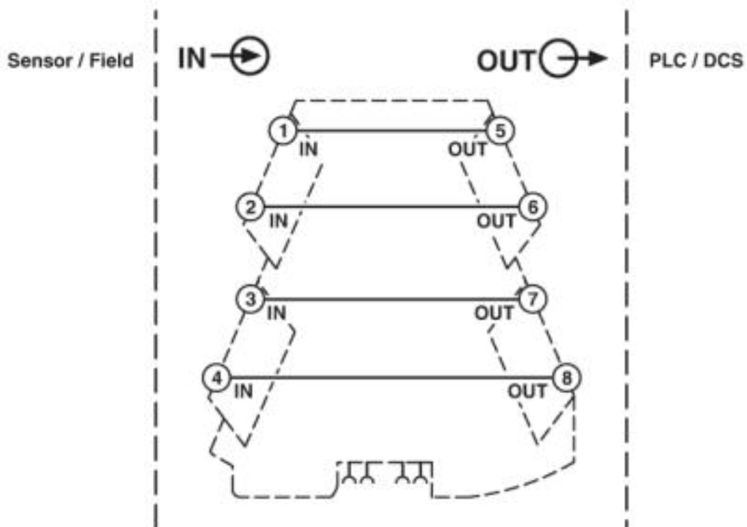
Block diagram
