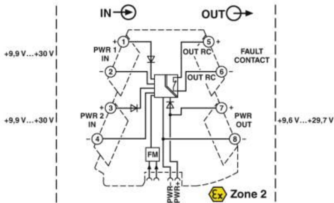
Block diagram
