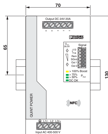
Dimensional drawing
