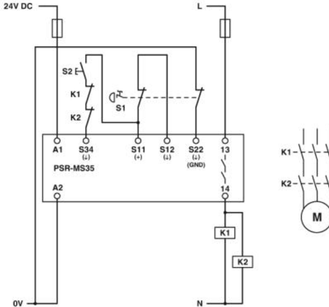
Application drawing
