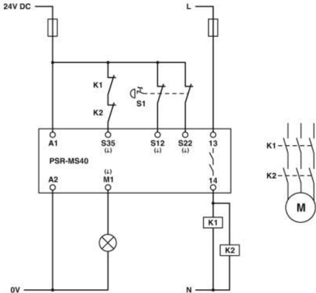
Circuit diagram
