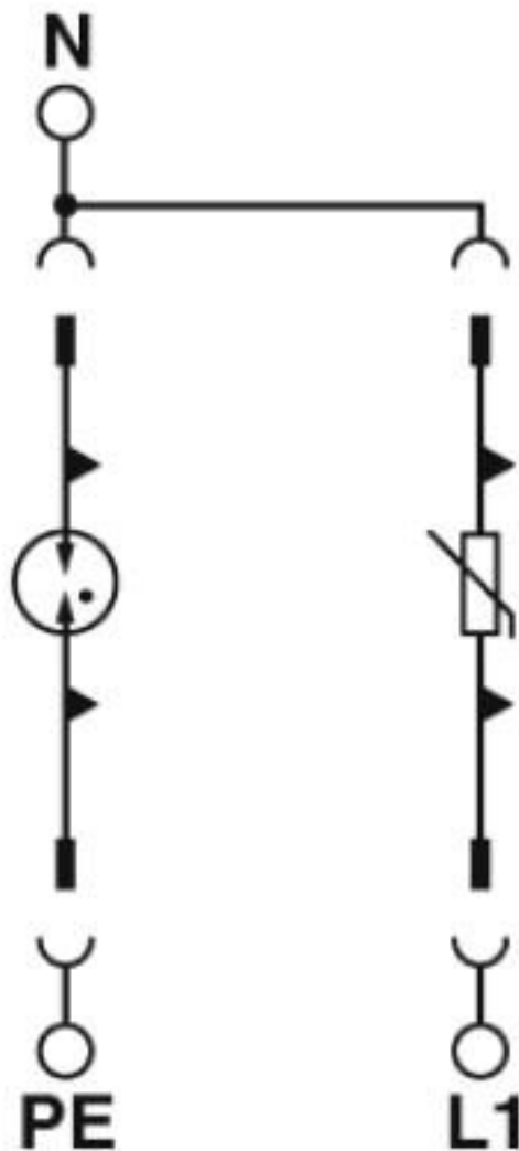
Circuit diagram
