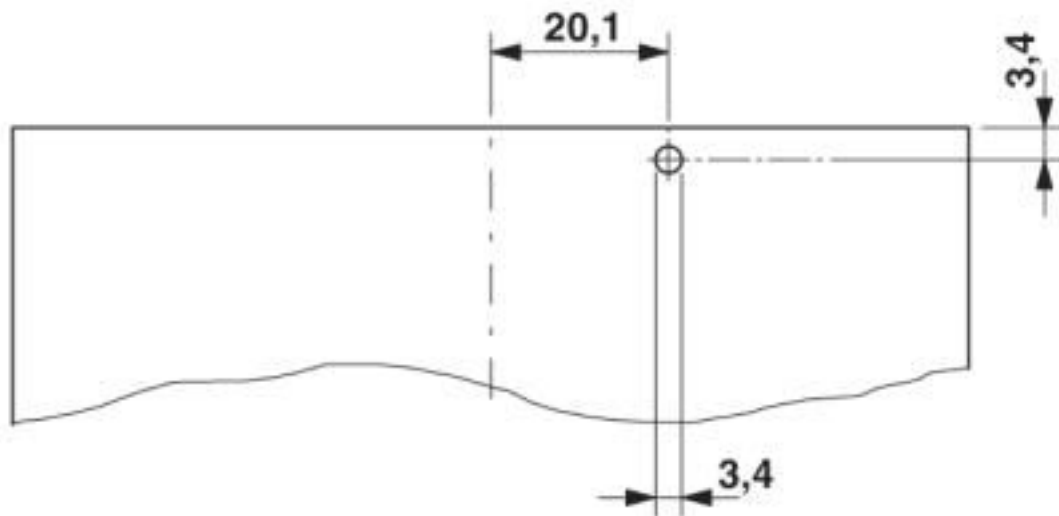
Drilling diagram
