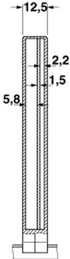
Dimensional drawing
