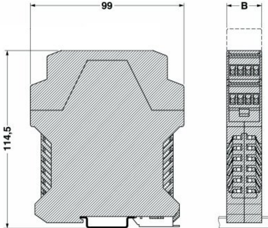
Dimensional drawing
