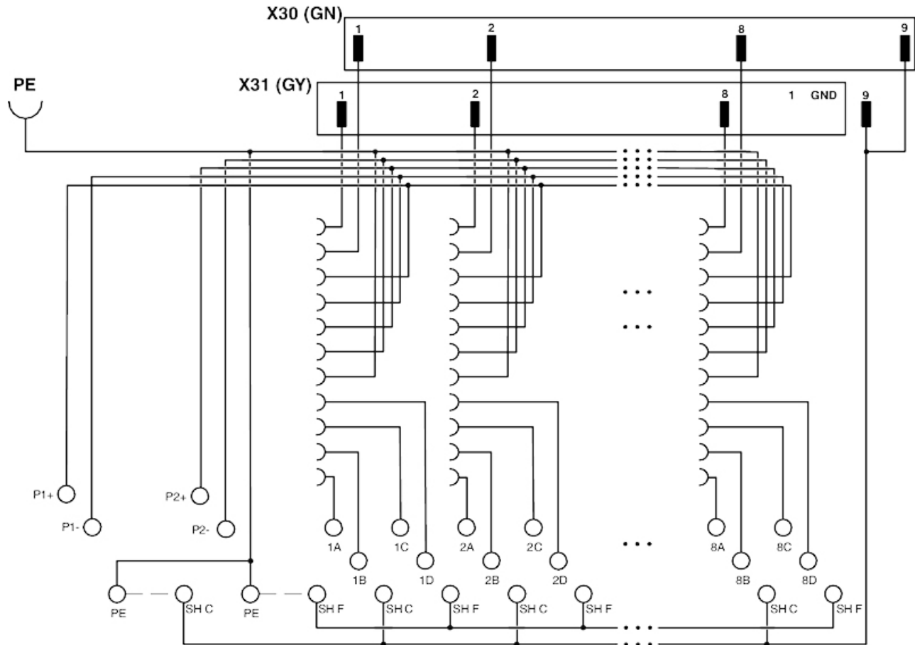
Circuit diagram
