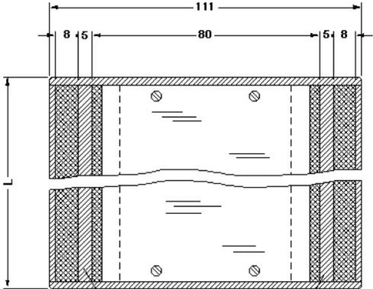
Dimensional drawing
