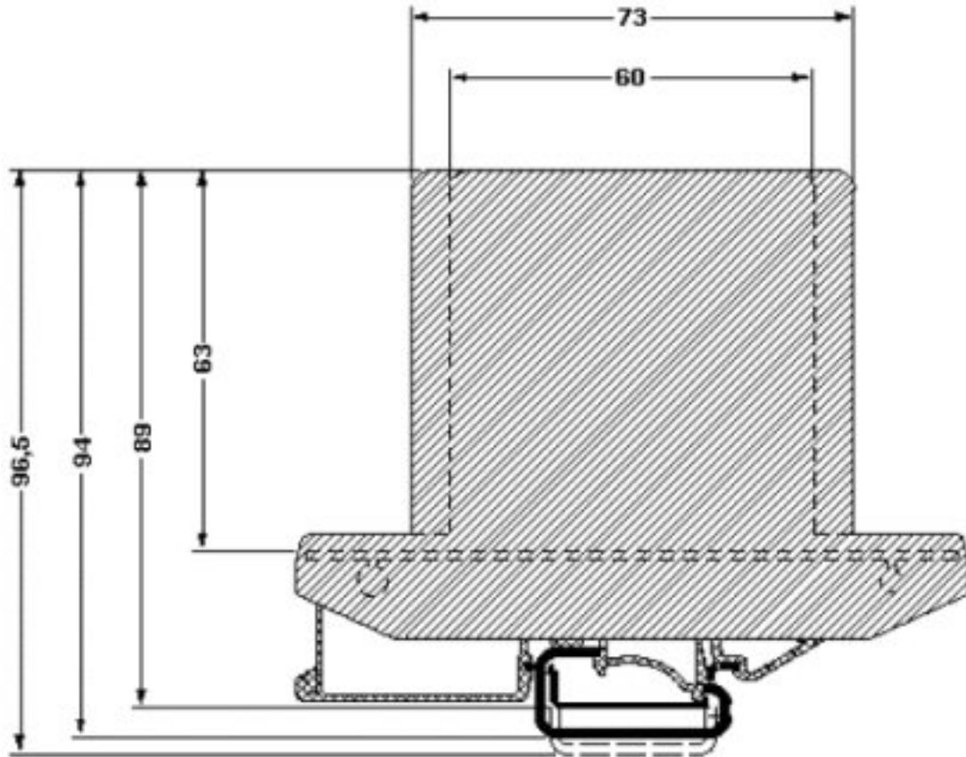
Dimensional drawing
