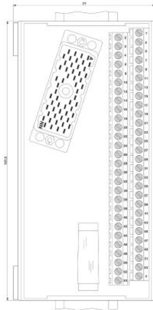
Dimensional drawing
