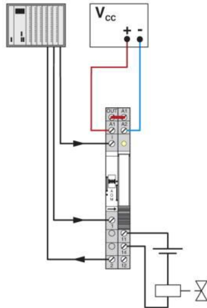
Application drawing
