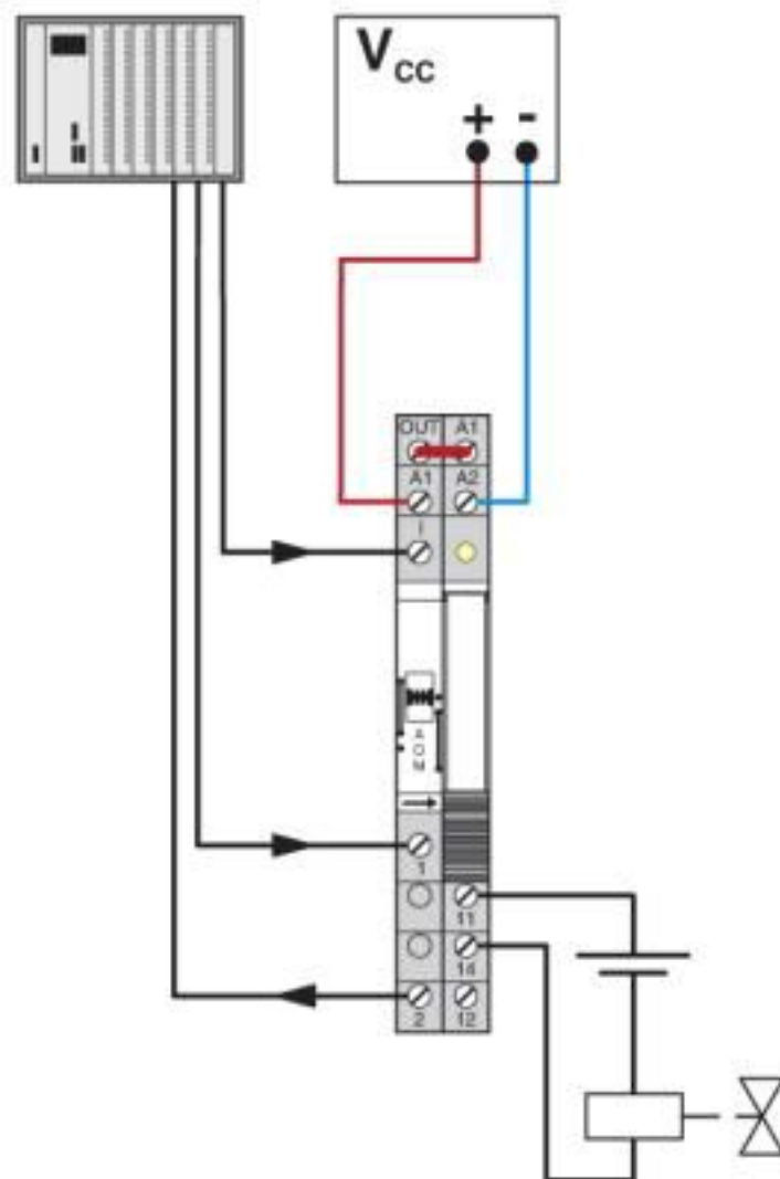
Application drawing
