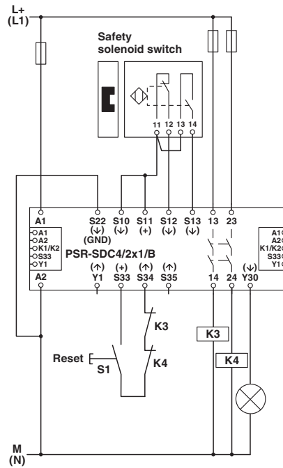
Circuit diagram
