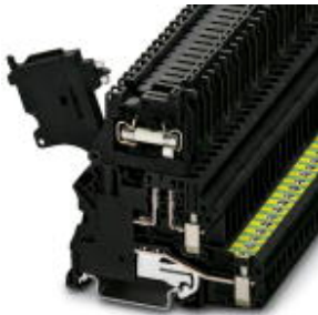
Lever-type fuse terminal block, color: black, for 5 x 20 mm G fuse inserts, with LED for 250 V AC
