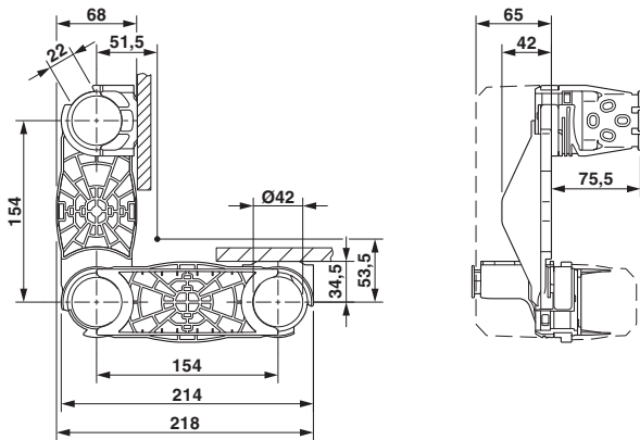
Dimensional drawing
