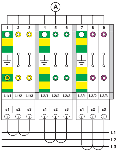
Connection diagram
