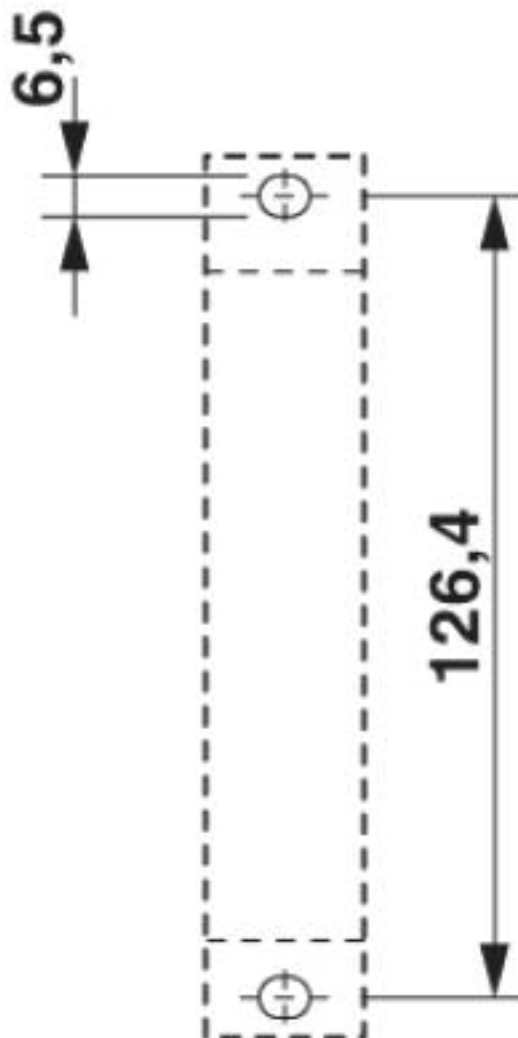
Dimensional drawing
