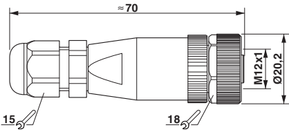
Dimensional drawing
