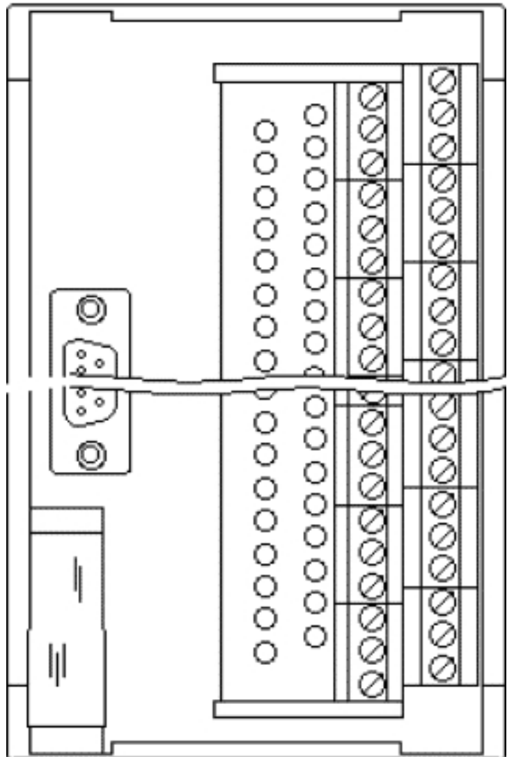
Schematic diagram
