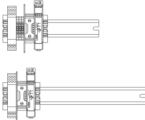
Application drawing
