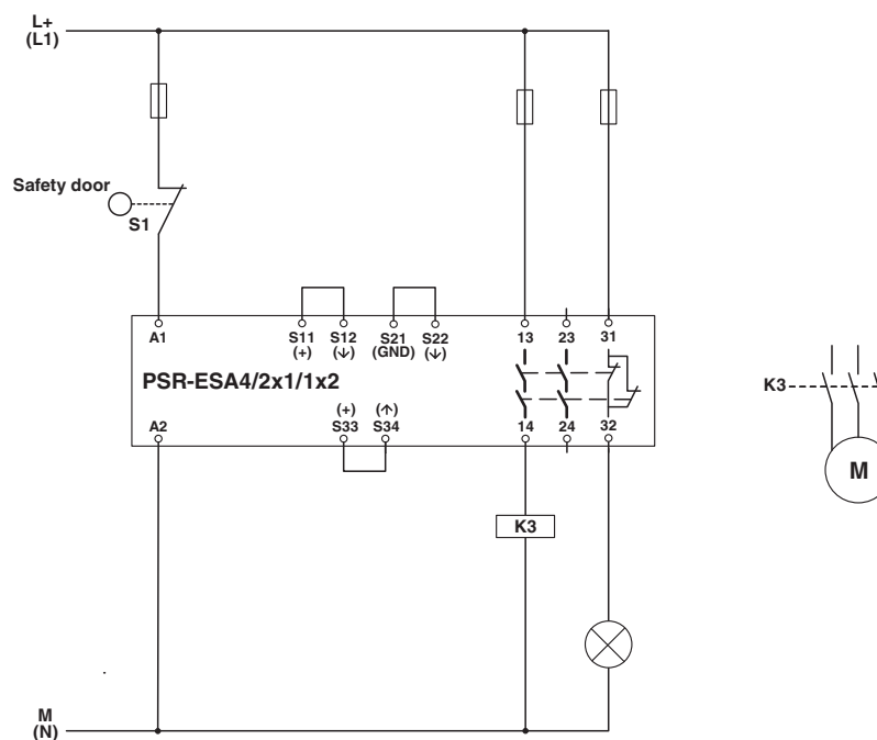
Circuit diagram
