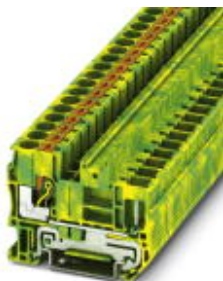
Ground modular terminal block, Connection method: Push-in / plug connection, Cross section: 0.5 mm 2 - 10 mm 2 , AWG: 20 - 8, Width: 8.2 mm, Color: green-yellow, Mounting type: NS 35/7,5, NS 35/15
