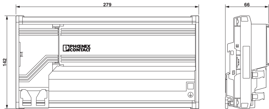
Dimensional drawing
