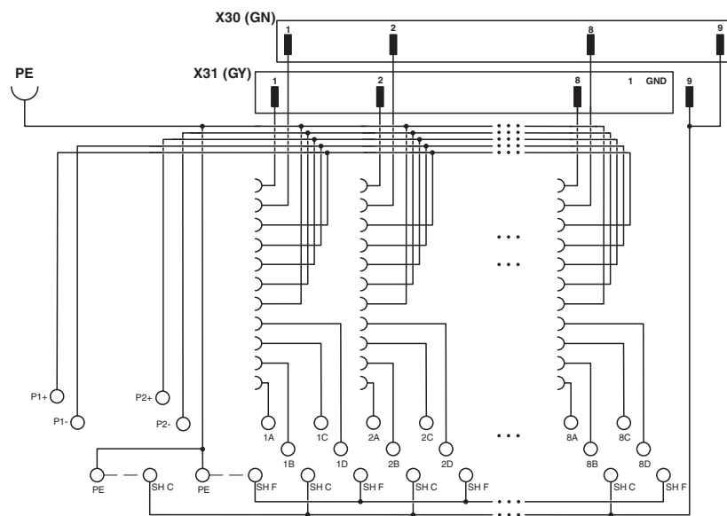
Circuit diagram
