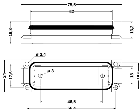
Dimensional drawing of panel mounting frame
