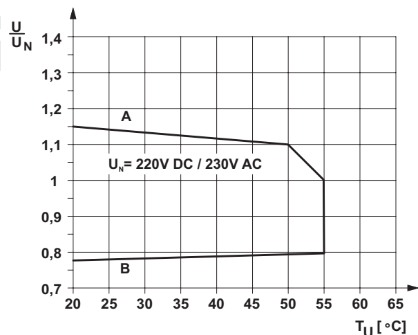
Figure 4 Operating voltage range for 230 V AC/DC
