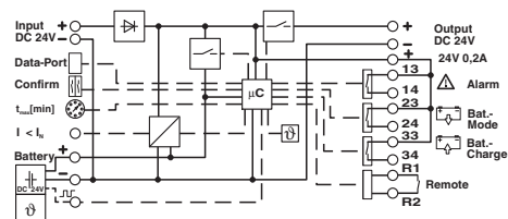
Block diagram
