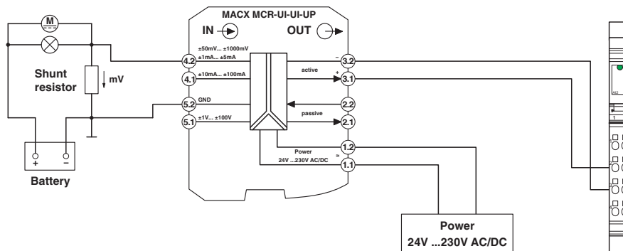
Application drawing
