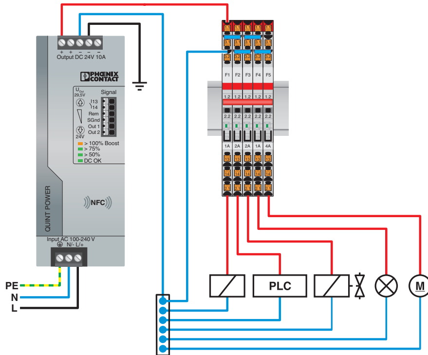
Application drawing
