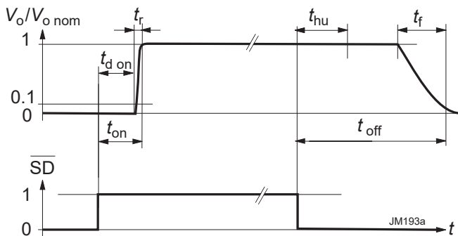
Fig. 4 Typical output response to the SD-signal.
