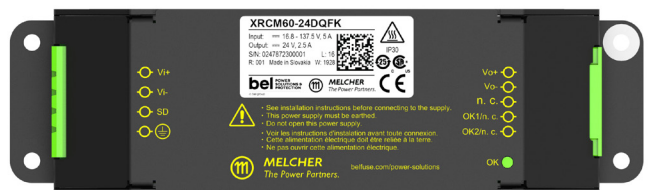
Fig. 12b Pin allocation of RCM60 (K option)
