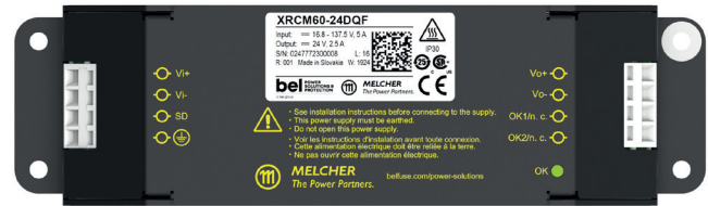
Fig. 11 Pin allocation of RCM60 (standard version)
