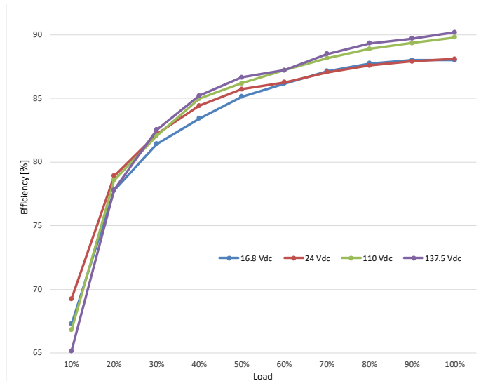
Fig. 3 Efficiency versus V_i and P_o (XRCM60-24DQF)
