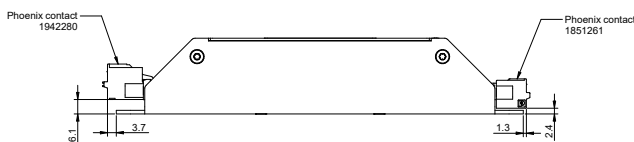
Fig. 12a Assembled input and output connector RCM60 (K option)
