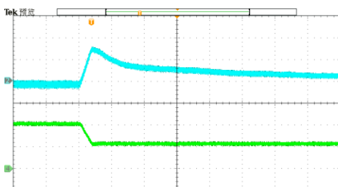
Figure 15. Load Transient V1, 203 to 101.5 A, 1A/μs (200 μs/div) CH2: V 1 (200mV/div) CH4: I 1 (100A/div)
