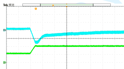
Figure 16. Load Transient V1, 101.5 to 203 A, 1A/μs (200 μs/div) CH2: V 1 (200mV/div) CH4: I 1 (100A/div)
