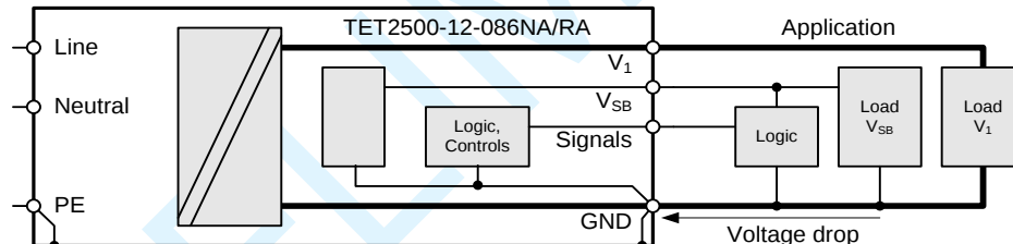
Figure 21. Common Low Impedance Ground Plane
