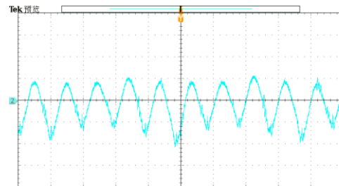
Figure 12. V_i Ripple 230VAC, full load (2us/div)
