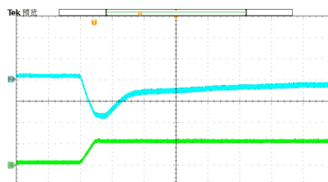
Figure 14. Load Transient V1, 10.15 to 111.65 A, 1A/μs (200 μs/div) CH2: V 1 (200mV/div) CH4: I 1 (100A/div)
