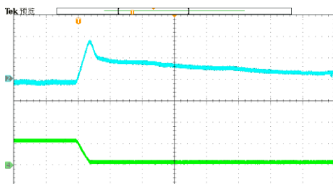
Figure 13. Load Transient V1, 111.65 to 10.15 A, 1A/μs (200 μs/div) CH2: V 1 (200mV/div) CH4: I 1 (100A/div)
