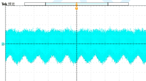
Figure 11. V_i Ripple 230VAC, full load (10ms/div)
