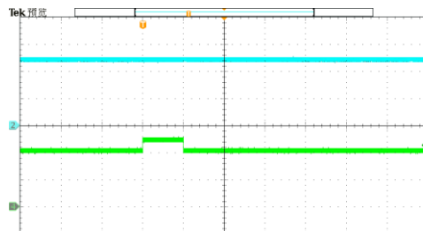
Figure 20. Short circuit on V1 (20ms/Div) CH2: V 1 (5V/div) CH4: V in (100A/div)
