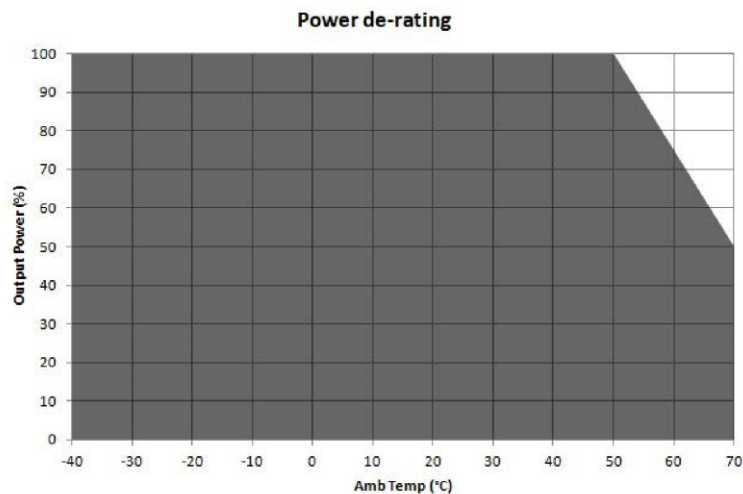
Figure 1. Derating Curve for all Outputs
