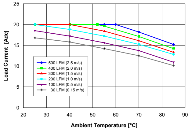
Fig. 1 : Available load current vs. ambient air temperature and airflow rates for converter with G height pins mounted vertically with air flowing from pin 1 to pin 3, MOSFET temperature \leq 125\text{ }^{\circ}\text{C} , V_{in} = 48\text{ V} .
