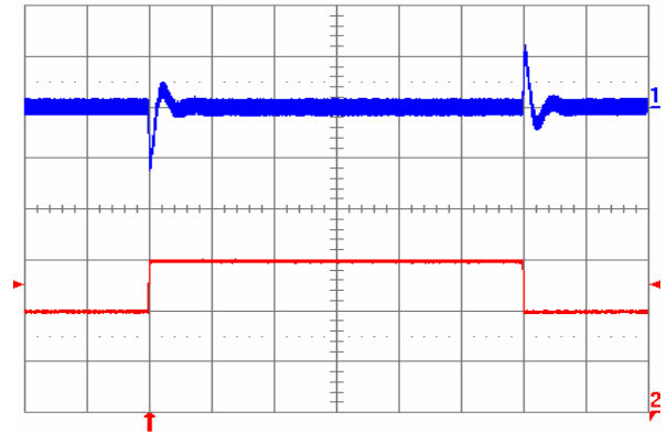
Fig. 10: Output voltage response to load current step-change (10 A – 15 A – 10 A) at V_{in} = 48 V. Top trace: output voltage (100 mV/div.). Bottom trace: load current (5 A/div.). Current slew rate: 5 A/ \mu s. C_o = 470 \mu F POS + 1 \mu F ceramic. Time scale: 0.2 ms/div.
