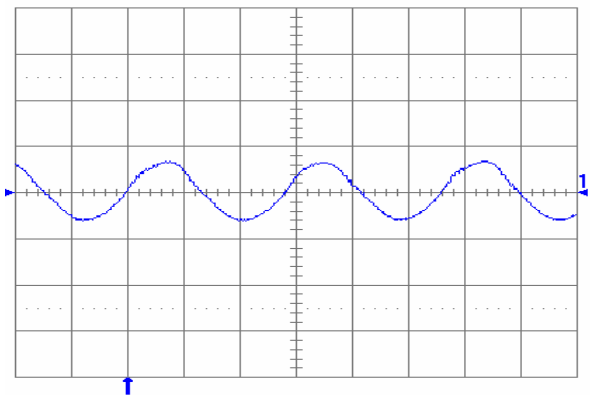
Fig. 11: Output voltage ripple (50 mV/div.) at full rated load current into a resistive load with C_o = 10 \mu F tantalum + 1 \mu F ceramic and V_{in} = 48 V. Time scale: 1 \mu s/div.
