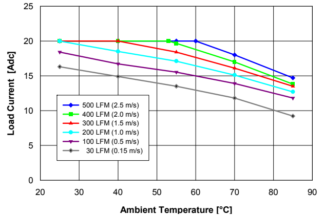
Fig. 2: Available load current vs. ambient air temperature and airflow rates for converter with G height pins mounted horizontally with air flowing from pin 1 to pin 3, MOSFET temperature \leq 125\text{ }^{\circ}\text{C} , V_{in} = 48\text{ V} .
