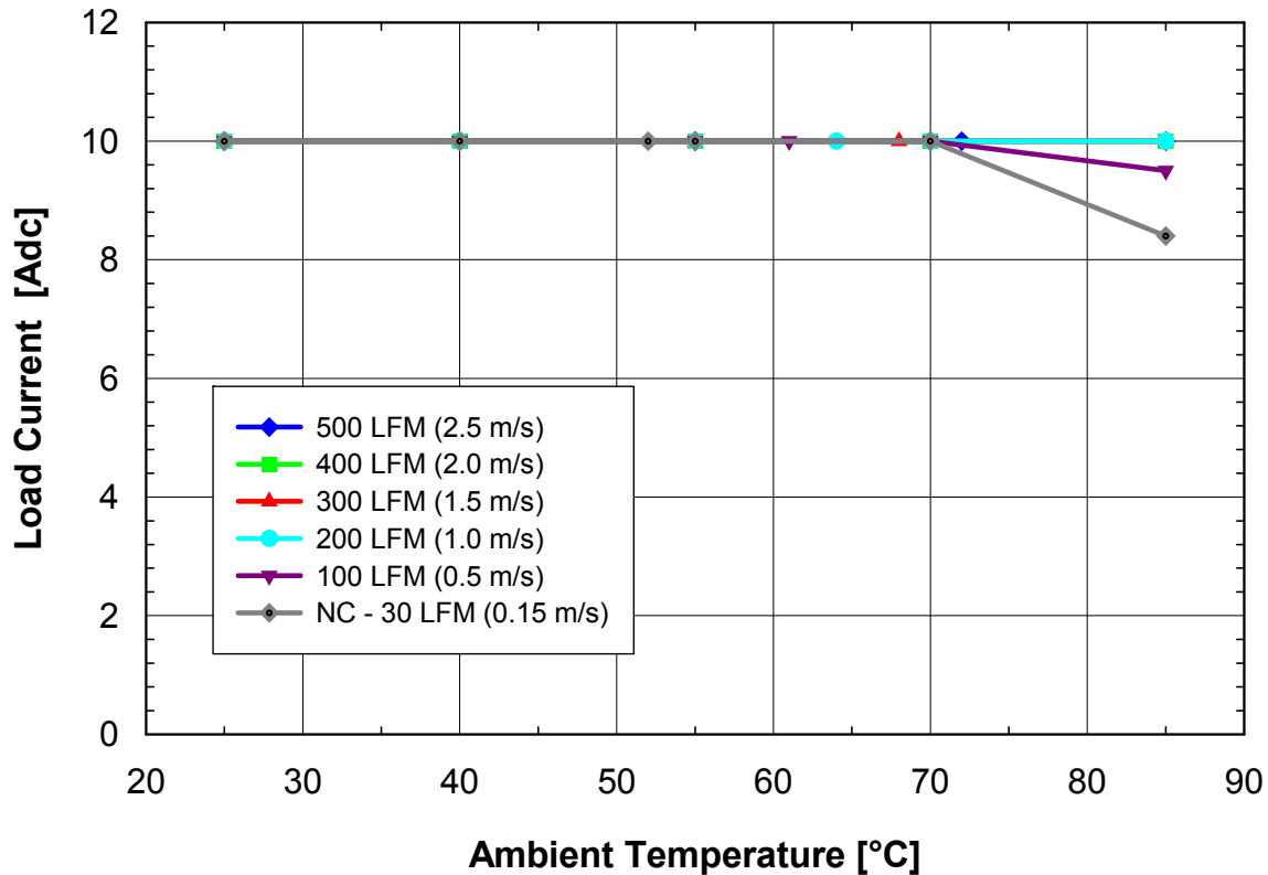
Figure 1. Available load current vs. ambient air temperature and airflow rates for SSQE48T10033 converter mounted vertically with air flowing from pin 1 to pin 3, V_{in} = 48 V. Note: NC – Natural convection
