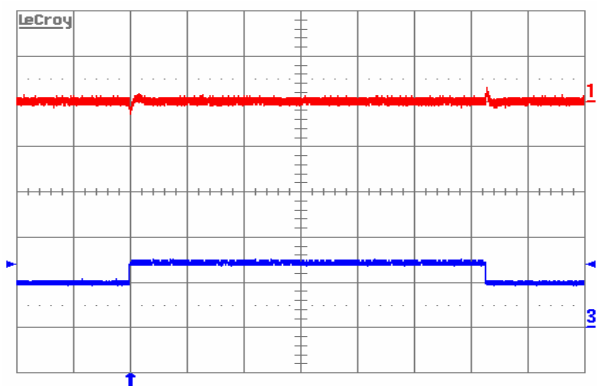
Figure 9. Output voltage response to load current step-change (5A-7.5A-5A) at V_{in}=48\text{ V} . Top trace: output voltage (100 mV/div.). Bottom trace: load current (5A/div.). Current slew rate: 5A/ \mu\text{s} . C_o=470\mu\text{F} POS + 1 \mu\text{F} ceramic. Time scale: 0.2 ms/div.
