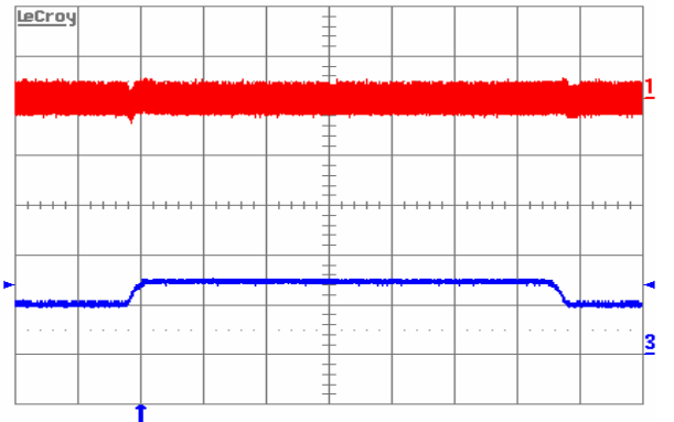
Figure 8. Output voltage response to load current step-change (5A-7.5A-5A) at V_{in}=48\text{ V} . Top trace: output voltage (50 mV/div.). Bottom trace: load current (5A/div.). Current slew rate: 0.1A/ \mu\text{s} . C_o=1\mu\text{F} ceramic + 10 \mu\text{F} tantalum. Time scale: 0.2ms/div.
