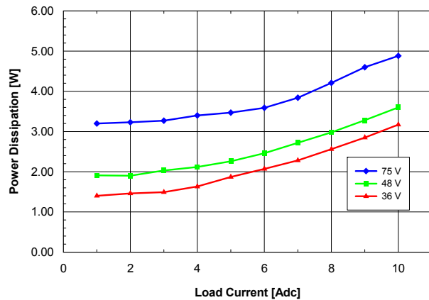
Figure 4. Power dissipation vs. load current and input voltage for SSQE48T10033 converter mounted vertically with air flowing from pin 1 to pin 3 at a rate of 300 LFM (1.5 m/s) and T_a = 25^\circ\text{C} .
