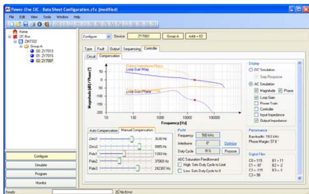
Figure 45. PWM Controller Window
