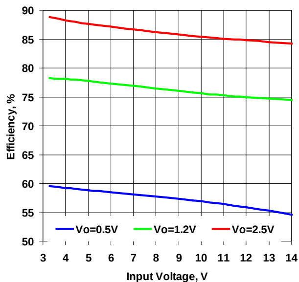
Figure 7. Efficiency vs. Input Voltage, I_{out}=7A , F_{sw}=500kHz
