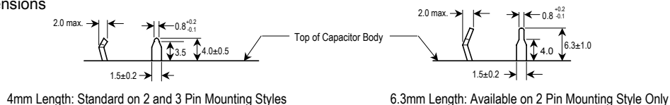
Pin Dimensions
