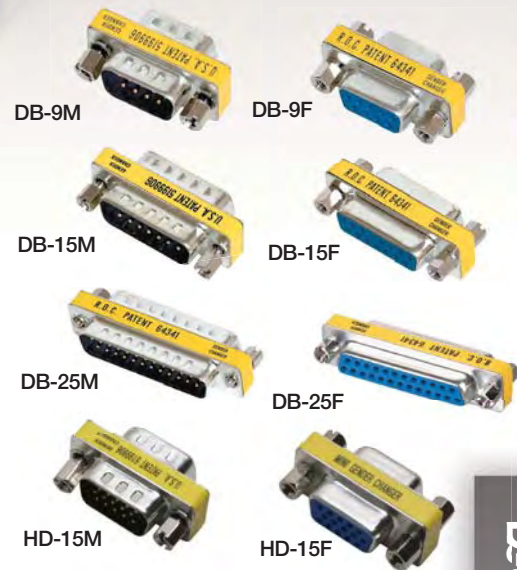
Fig.1 D-Sub Slim Line Adapters
