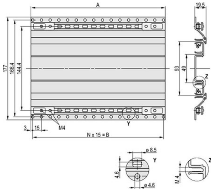
Extruded side panel
