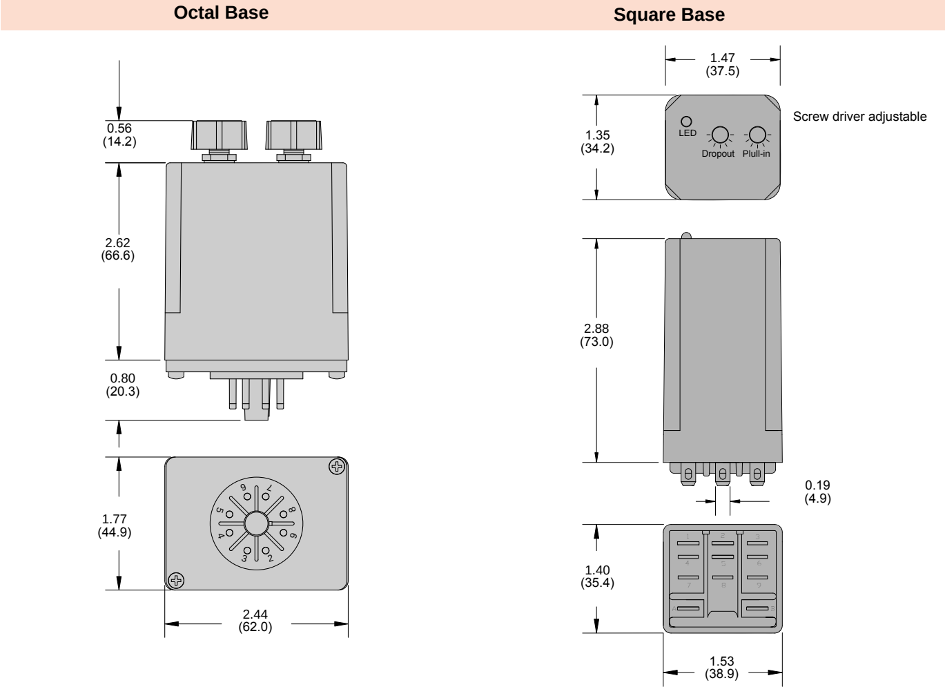
Outline Dimensions Dimensions Shown in inches & (millimeters)
