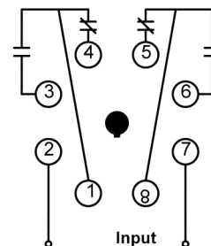
Octal Base
