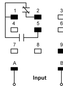
Square Base
