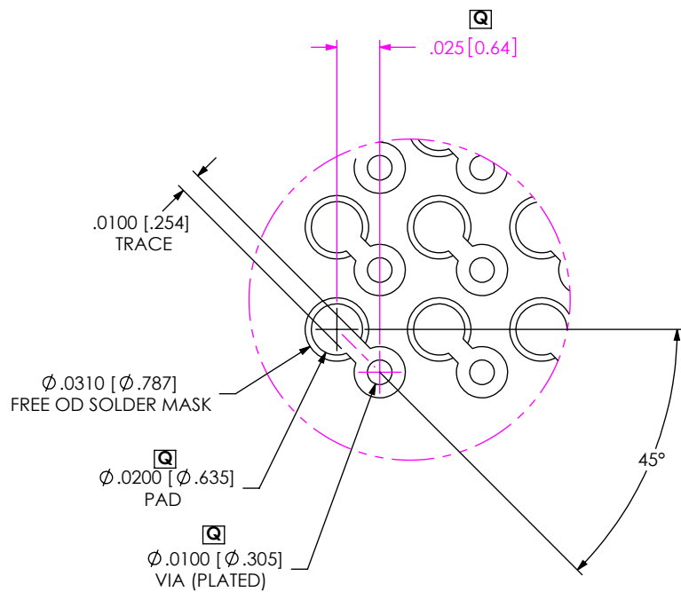
DETAIL 'B'
