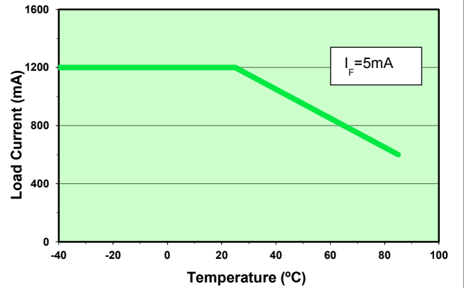
Figure 2: Maximum Load Current vs. Temperature
