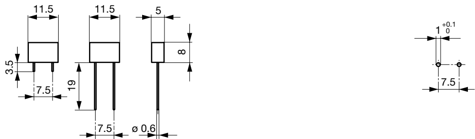
Drilling diagram
