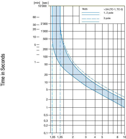
Multiple of Rated Current I_n Reference Temperature +23°
