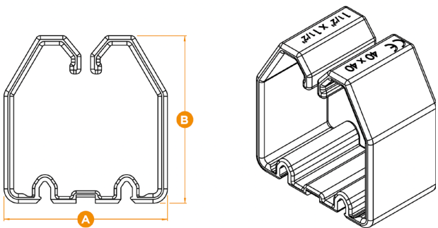
Wire retainer
