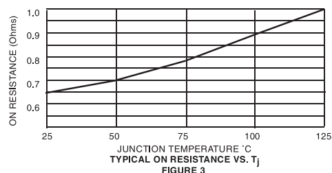
TYPICAL ON RESISTANCE VS. T j FIGURE 3
