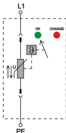
Circuit diagram
