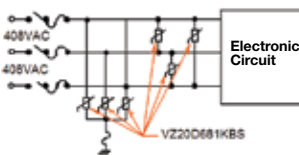
MOV for 3 Phase AC Line Protection
