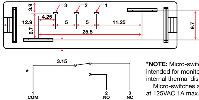
Micro-switch (BOTTOM)
