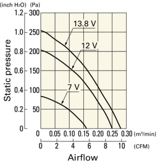
9BD12FC6-1 With pulse sensor
