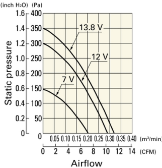
9BD12SC6-1 With pulse sensor
