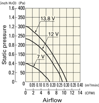
9BD12HC6-1 With pulse sensor
