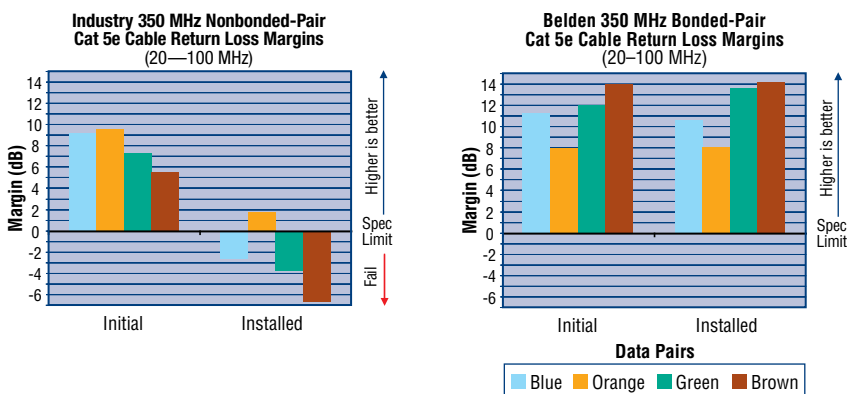
In an Installation Stress Test that simulates the installation process, the Cat 5e nonbonded-pair cables (left) showed an RL degradation of more than 12 dB. The Bonded-Pair cables (right) exhibited little change in RL performance.
